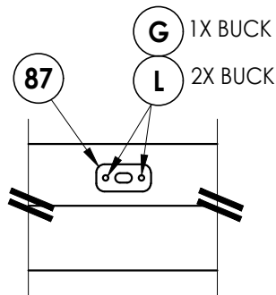
DETAIL 2
